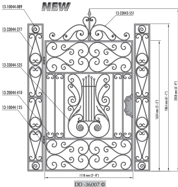
A. 13-33044-535 Forged steel DD 3/4" x 5/16" (20 mm x 8 mm or .7874" x .3149") Plain Flat Bar † 32-1/16" ↔ 20-7/8" ± 28.22 lbs
